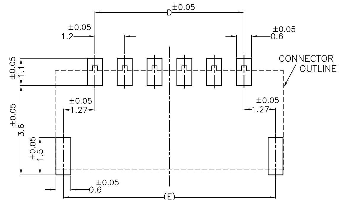
RECOMMENDED PCB PATTERN LAYOUT
