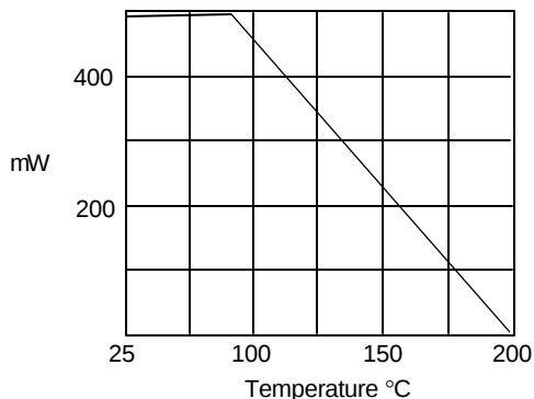
Figure 2 - Derating Curve
