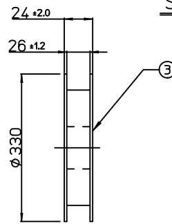
PLASTIC BOBBIN
