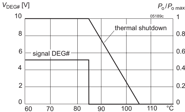
Fig. 9 Degradation signal V_{DEG\#} versus case temperature T_C
