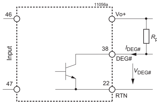
Fig. 8 Degradation signal: NPN output V_{DEG\#} \leq 40\text{ V} , I_{DEG\#} \leq 20\text{ mA}
