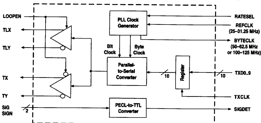
Figure 1. TQ9501 Transmitter
