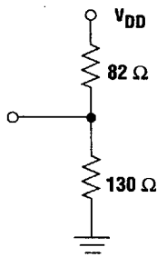
Figure 12c. PECL Test Load
