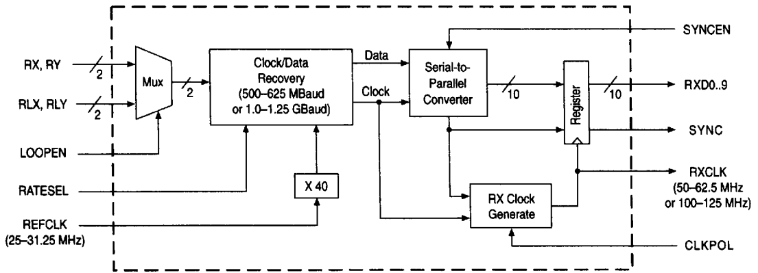
Figure 2. TQ9502 – Receiver
