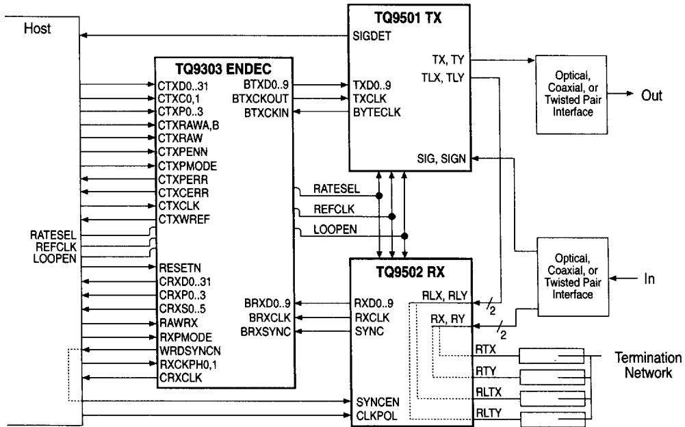
Figure 3. System Block Diagram – Fibre Channel
