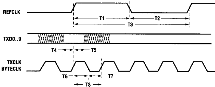
Figure 9. Serial Output Timing – TQ9501
