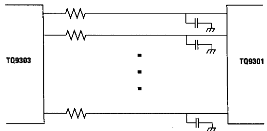
Figure 4. Adding resistance and capacitance to the TX data bus.
