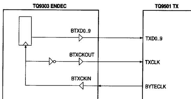
Figure 6. Transmitter Synchronization Circuit Block Diagram
