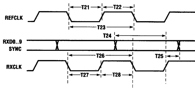
Figure 10. Bus Timing – TQ9502 Receiver
