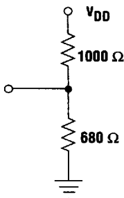
Figure 12a. TTL Test Load, RXCLK
