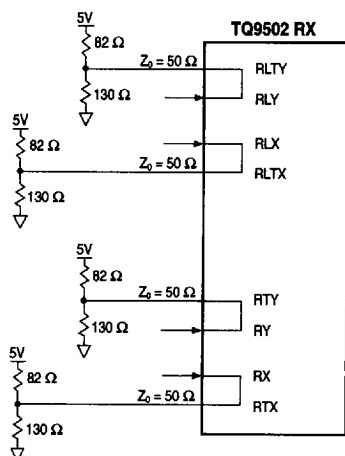
Figure 5. Fly-By™ Termination Schematic
