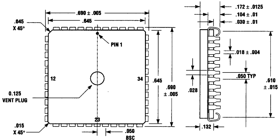
Figure 15. 44-Pin MQuad J-leaded Package
