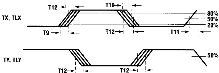
Figure 9. Serial Output Timing – TQ9501
