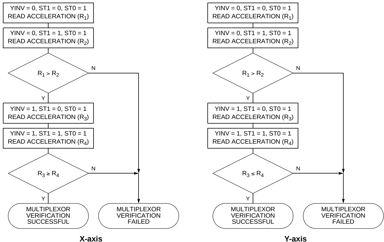
Figure 3-2 DSP Input Multiplexor Verification Flow Chart
