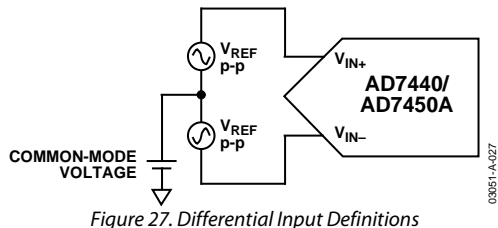
Figure 27. Differential Input Definitions
