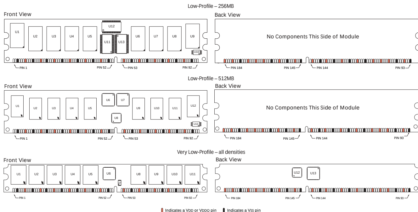
Figure 2: Pin Locations
