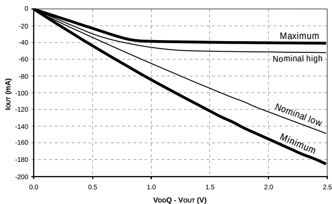
Figure 11: Pull-Up Characteristics
