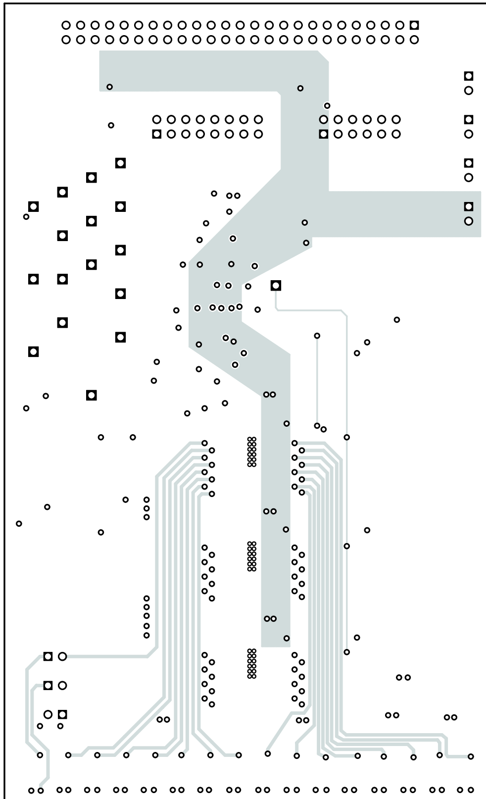
Figure 4. Layer 2 Routing
