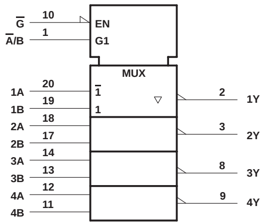
logic symbol†
