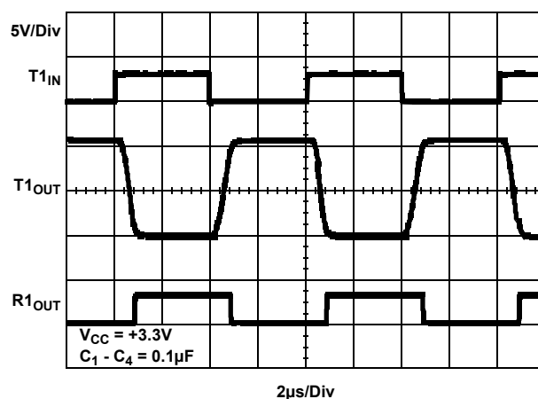
Figure 20. Loopback Test at 250kbps
