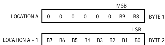
D_{OUT} from LTC1091 Stored in MC68HC05C4 RAM
