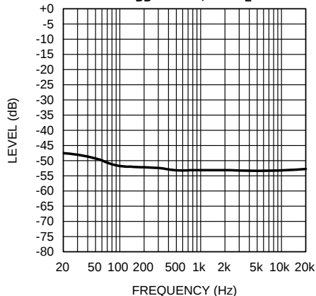
Figure 12. Input terminated with 10Ω
