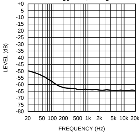
Figure 8. Input terminated with 10Ω
