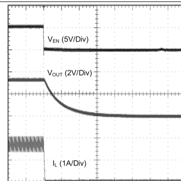
Figure 14. Shutdown Transient
