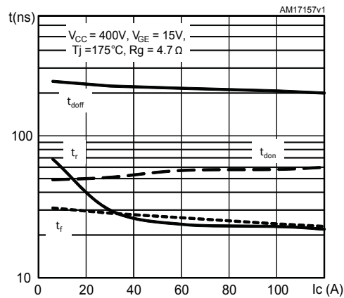
Figure 19. Switching times vs collector current
