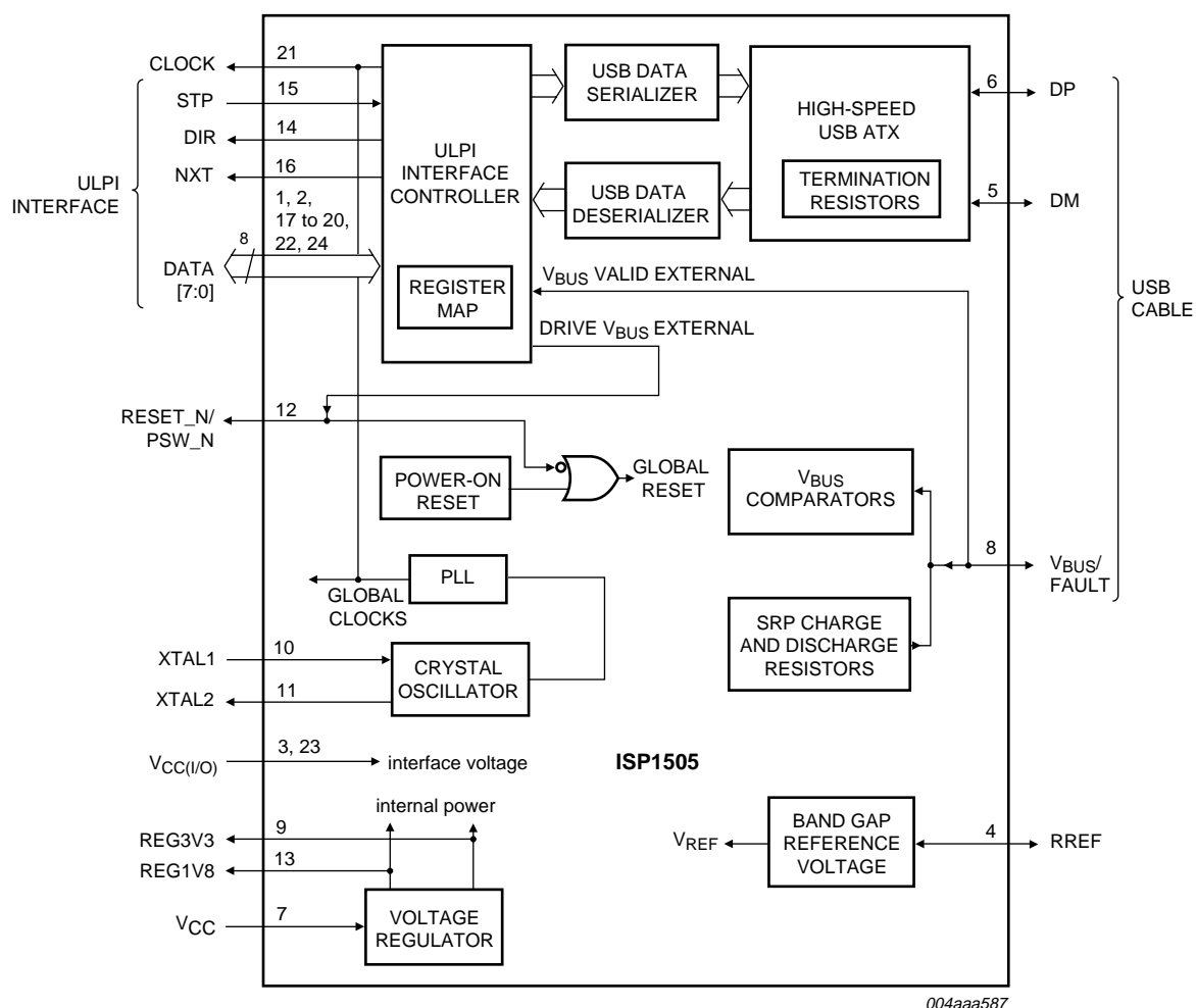
Fig 1. Block diagram
