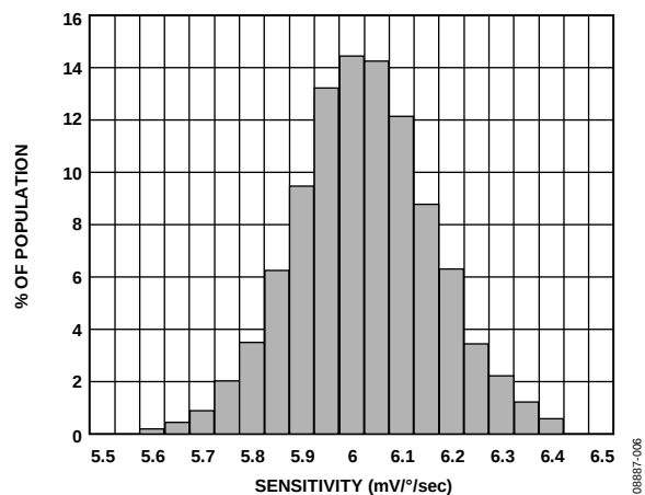
Figure 6. Sensitivity at 25°C ( V_{RATIO} = 5\text{ V} )
