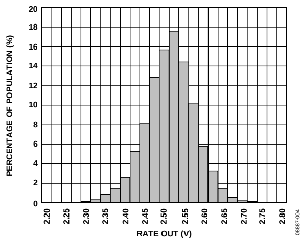
Figure 4. Null Output at 25°C ( V_{RATIO} = 5\text{ V} )
