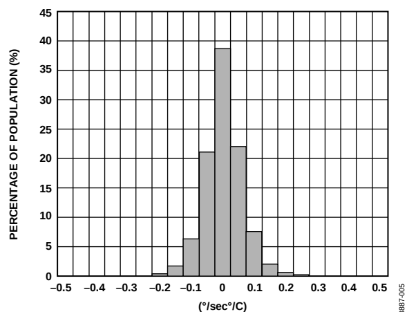
Figure 5. Null Drift over Temperature ( V_{RATIO} = 5\text{ V} )
