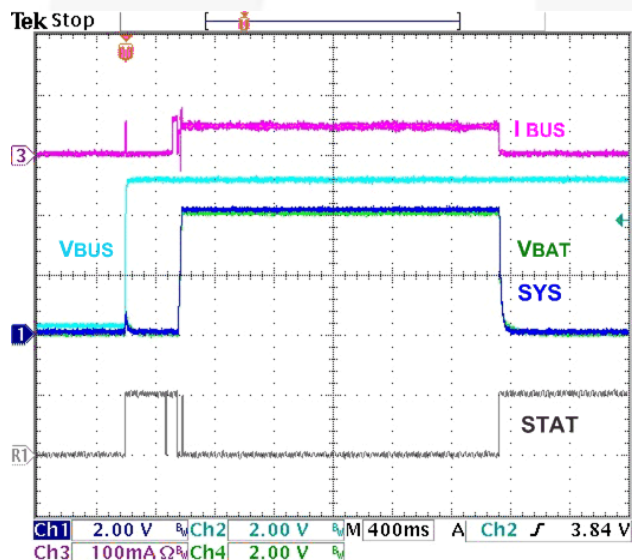
Figure 17. No Battery at V BUS Power-Up, FAN54040, 100 \Omega SYS Load, 1 k \Omega V BAT Load
