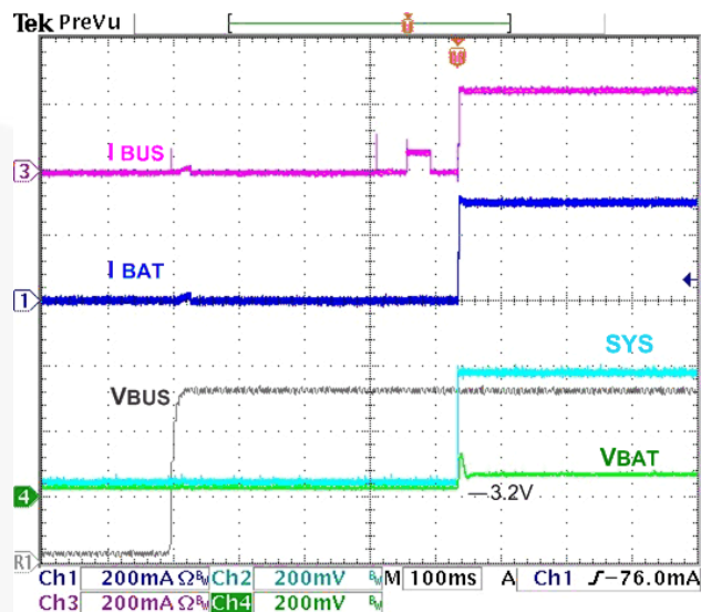
Figure 12. Charger Startup at V_{BUS} Plug-In, 500 mA I_{INBUSLIM} , 3.2 V _{BAT} , 100 \Omega SYS Load
