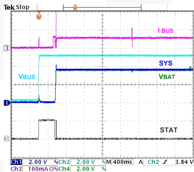
Figure 18. No Battery at V BUS Power-Up, FAN54042, 100 \Omega SYS Load, 1 k \Omega V BAT Load
