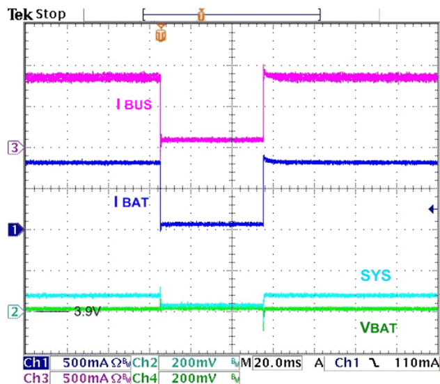
Figure 15. Battery Removal / Insertion while Charging, TE=0 , 3.9 V BAT , I_{CHRG}=950 mA, I_{BUSLIM}=\text{No Limit} , 50 \Omega SYS Load
