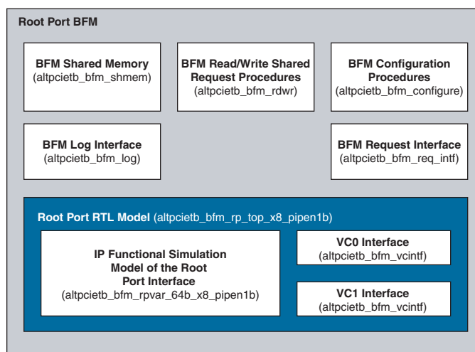
Figure 15–6. Root Port BFM
