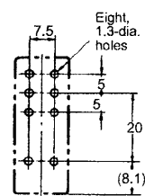
Mounting Holes
