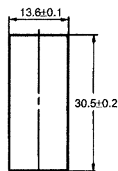
Panel Cutout
