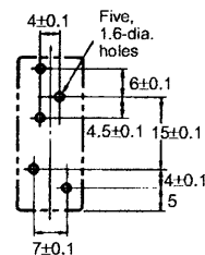
Mounting Holes
