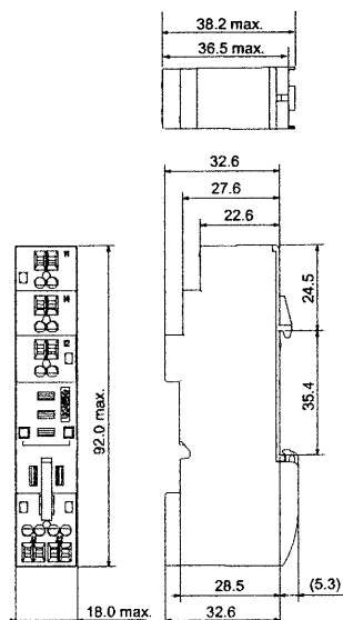
Option (with ejector and label attached)
