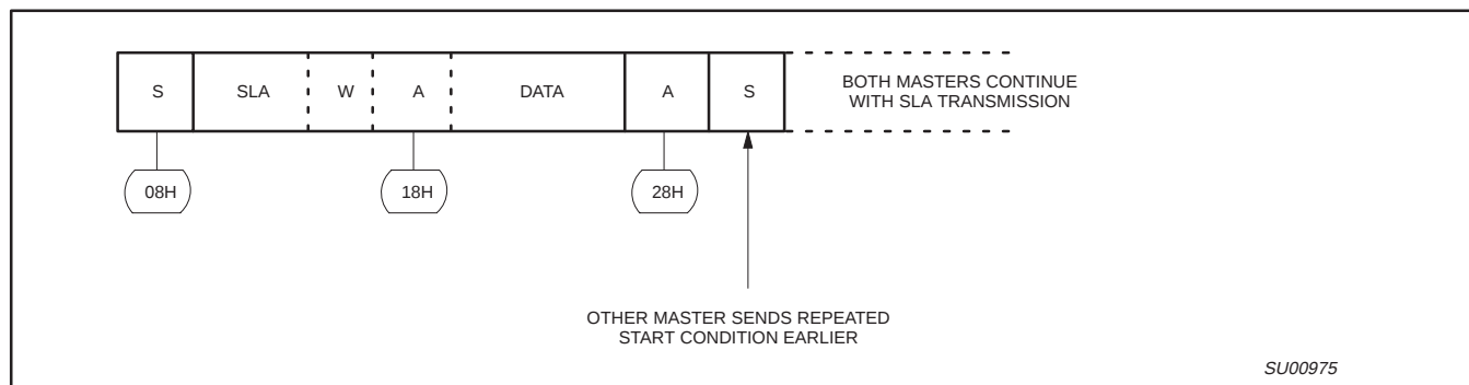
Figure 44. Simultaneous Repeated START Conditions from 2 Masters
