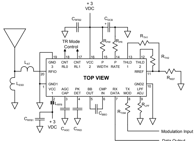
ASH Transceiver Application Circuit ASK Configuration
