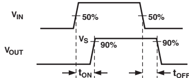
Test Circuit 4. Switching Times
