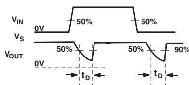
Test Circuit 5. Break-before-Make Time Delay, t_D
