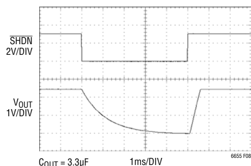
Figure 8. Shutdown Response with 5mA Source Load
