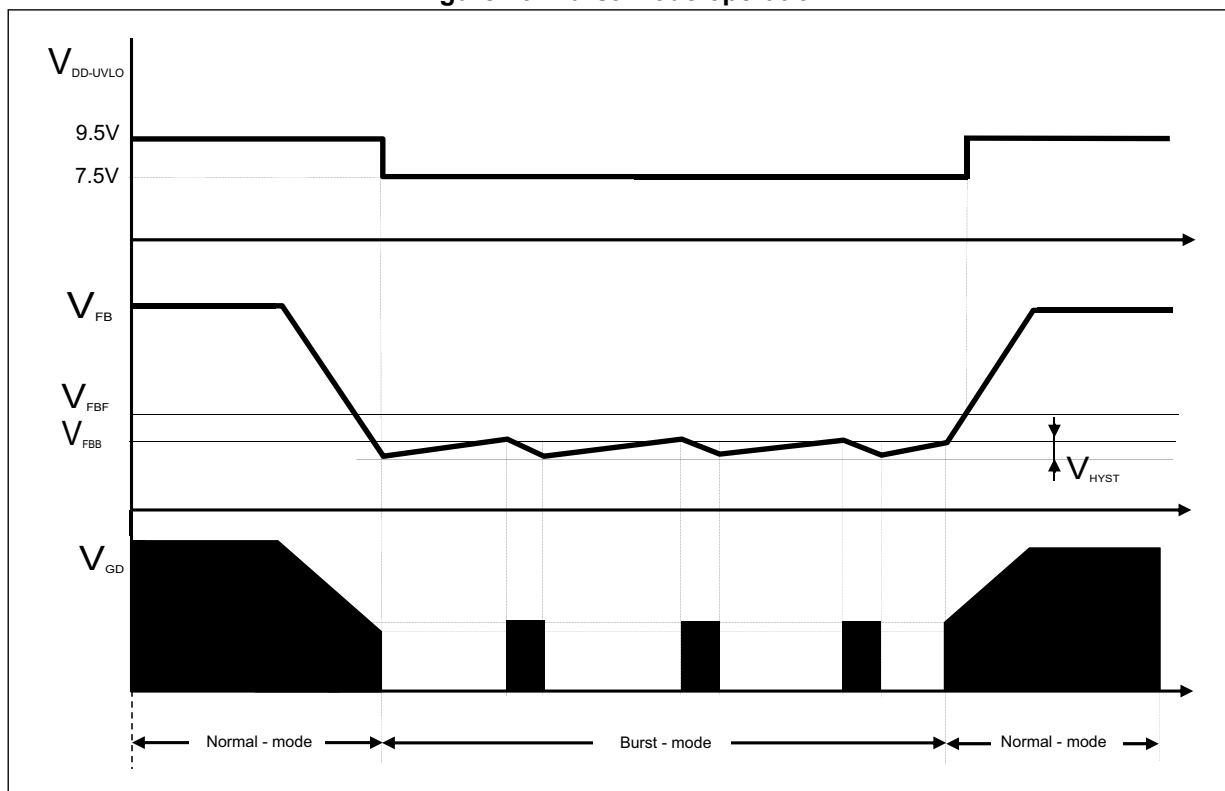
Figure 10. Burst-mode operation
