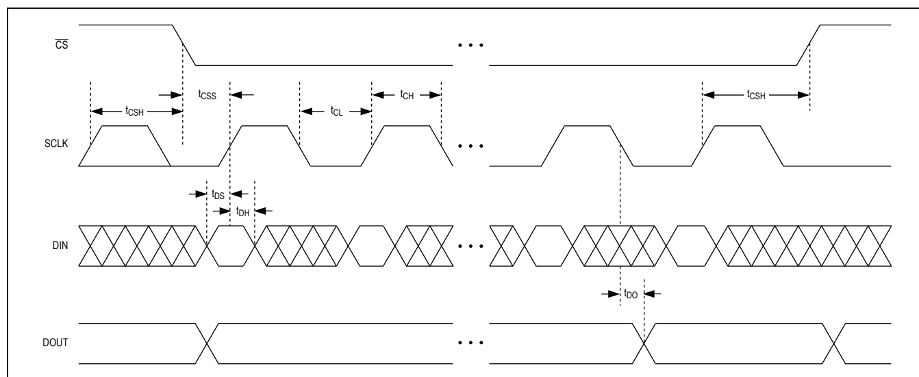
Figure 2. 4-Wire Interface
