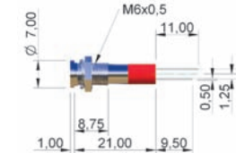
PINS
