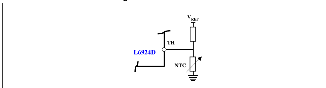
Figure 21. Pin connection
