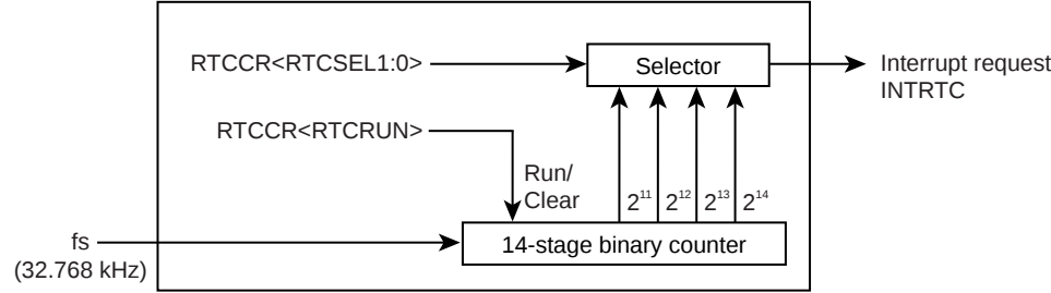
Figure 12-1 Block Diagram for Special Timer for CLOCK
