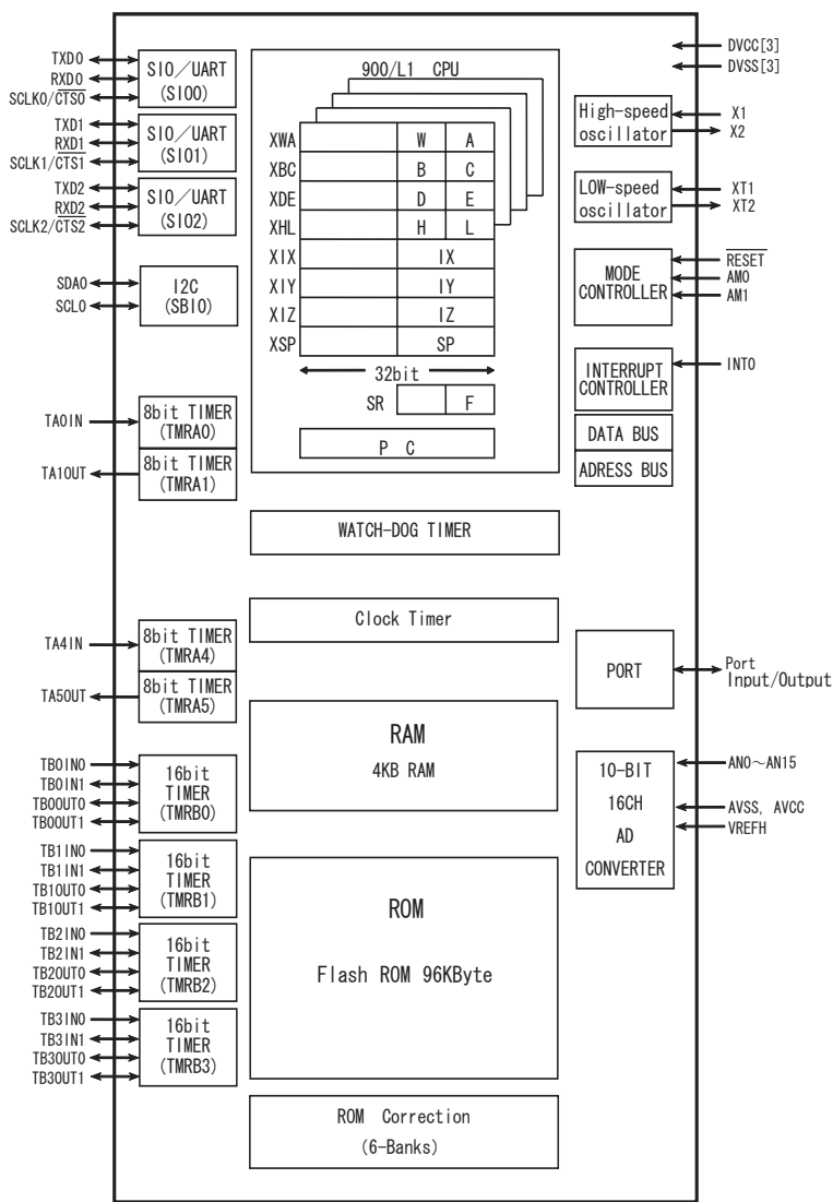
Figure 1-3 Block Diagram
