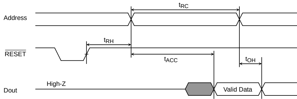
Figure 4.6.8 Read Timings After \overline{RESET}
