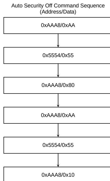
Figure 3.4.10 Auto Security Off Operation
