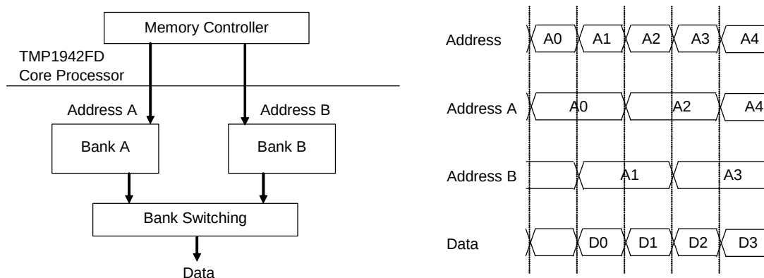
Figure 3.2.4 Interleave Configuration
