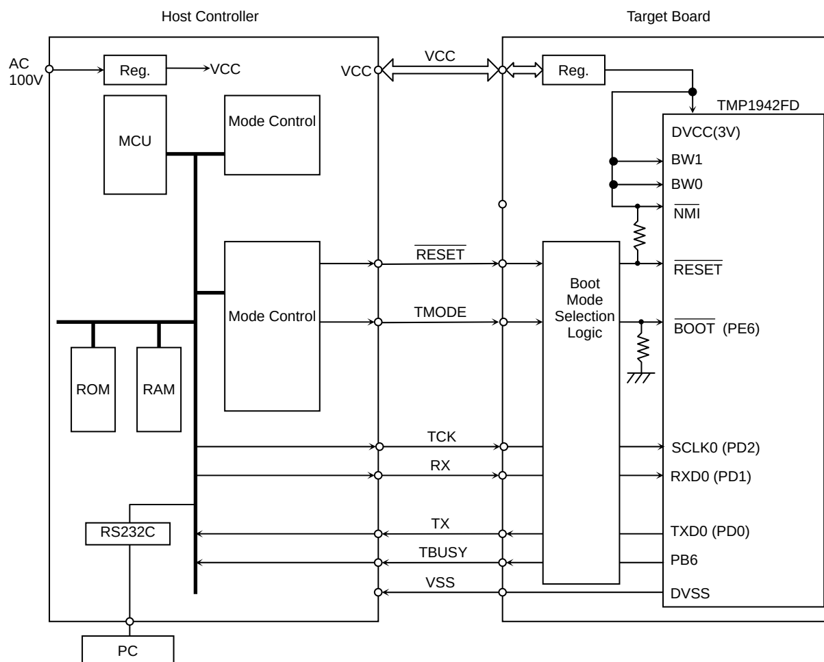
Figure 3.3.2 Example of a Connection between a Host Controller and a Target Board (When the SIO0 is Configured for I/O Interface Mode)
