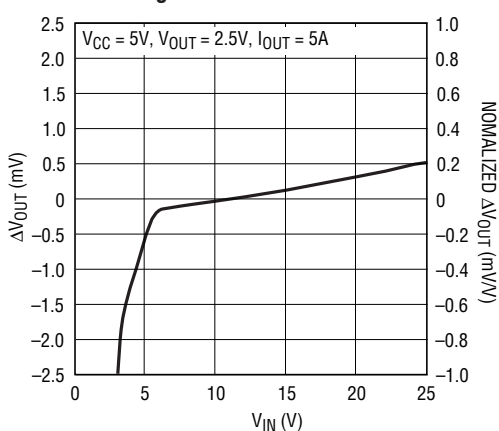
Line Regulation
