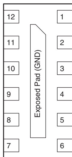
DFN-12 (Bottom View)
