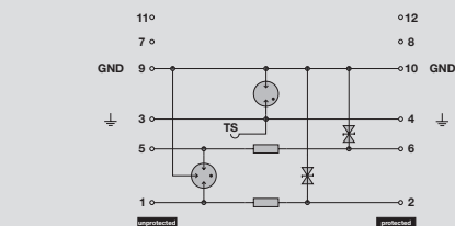
Complete module, floating ground
