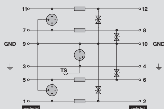
Complete module, floating around
