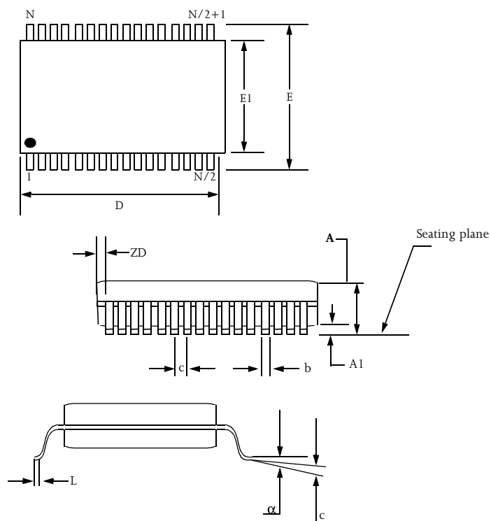
32-pin TSOP II
