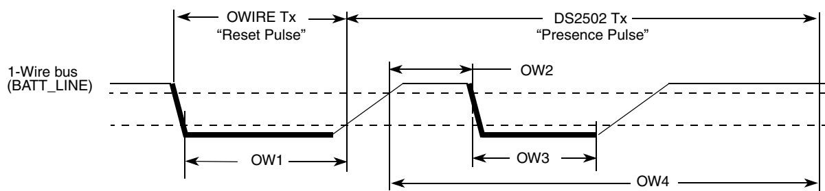
Figure 7. Reset and Presence Pulses (RPP) Timing Diagram
