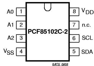
Fig.2 Pin configuration PCF85102C-2.
