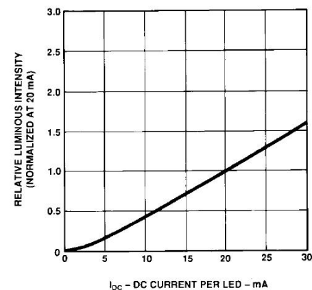
Figure 10: Relative Luminous Intensity vs. Forward Current
