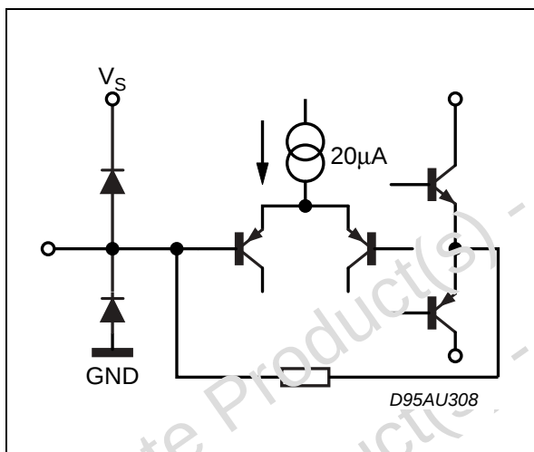
Figure 24. PIN: REARIN
