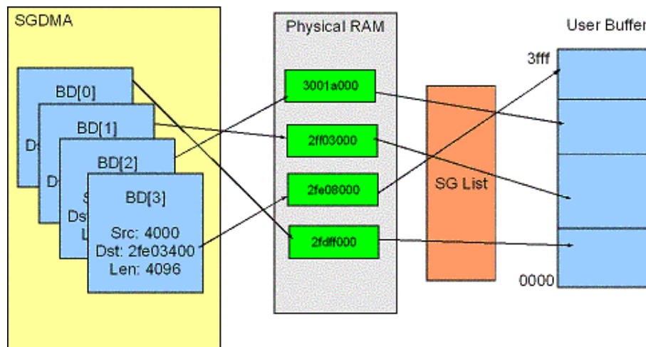
Figure 14: SGDMA Buffer Address Mapping
