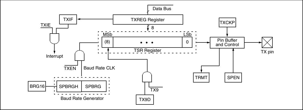
FIGURE 18-4: ASYNCHRONOUS TRANSMISSION, TXCKP = 0 (TX NOT INVERTED)
