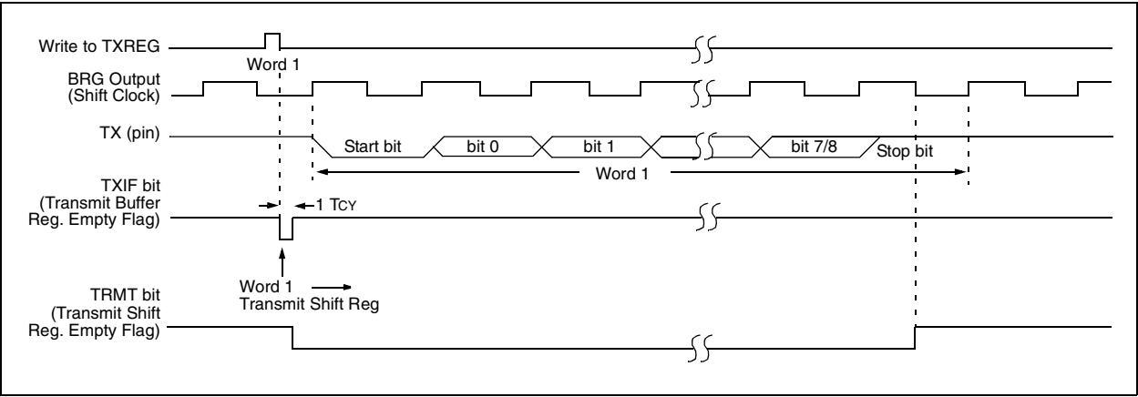
FIGURE 18-5: ASYNCHRONOUS TRANSMISSION (BACK TO BACK), TXCKP = 0 (TX NOT INVERTED)
