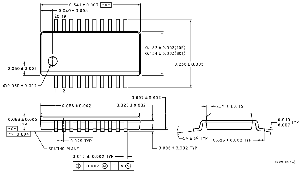
20-Lead (0.150" Wide) Shrink Small Outline Package, JEDEC Package Number MQA20
