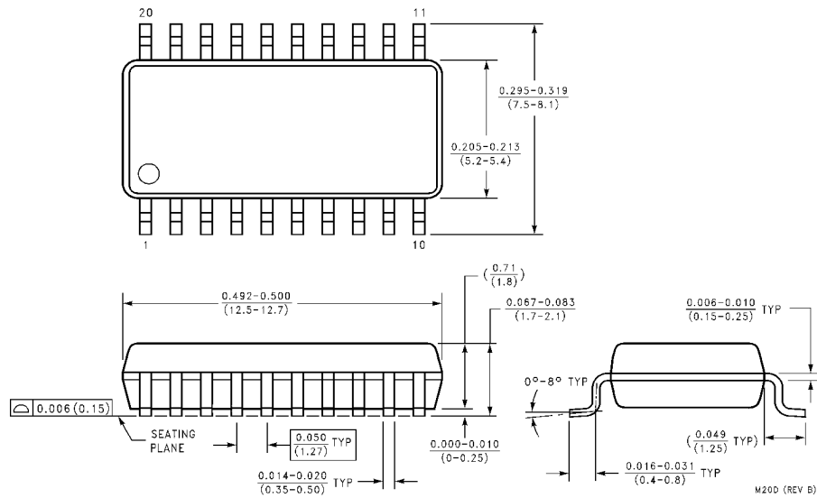
20-Lead Small Output Package-EIAJ (SJ) Order Number DM74ALS245ASJ Package Number M20D
