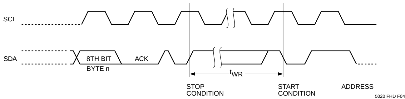
Figure 3. Start/Stop Timing
