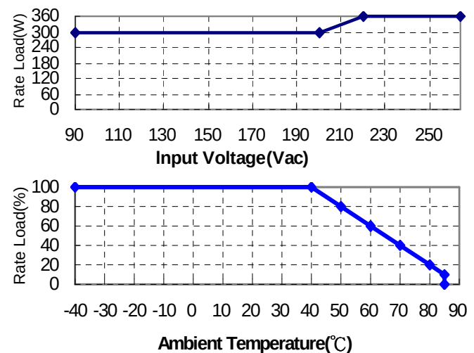
360W With Baseplate Cooled
