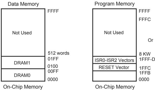
Figure 18. Memory Map
