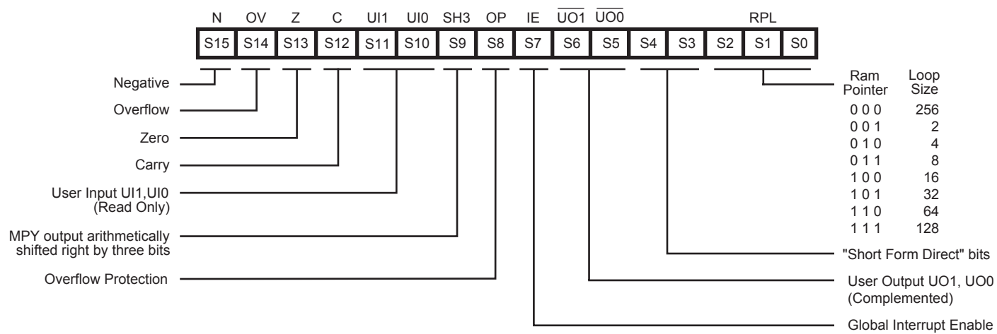
Figure 19. Status Register
