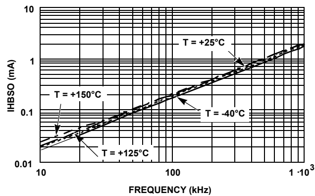
FIGURE 8. IHB OPERATING CURRENT vs FREQUENCY
