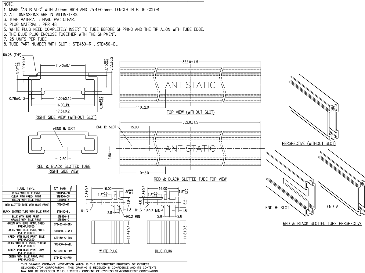
Figure 14. 28-pin SSOP, 32-pin SOIC (450 Mils Body) Shipping Tube, 51-51029
