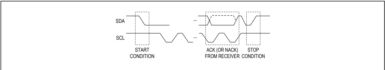
Figure 6. Start, Stop, and ACK Signals
