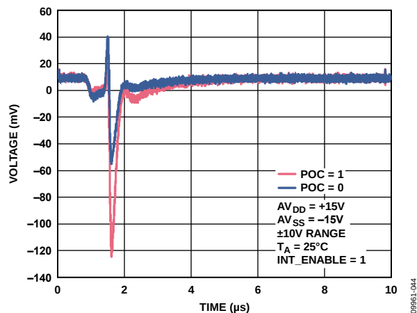
Figure 30. Voltage vs. Time on Output Enable
