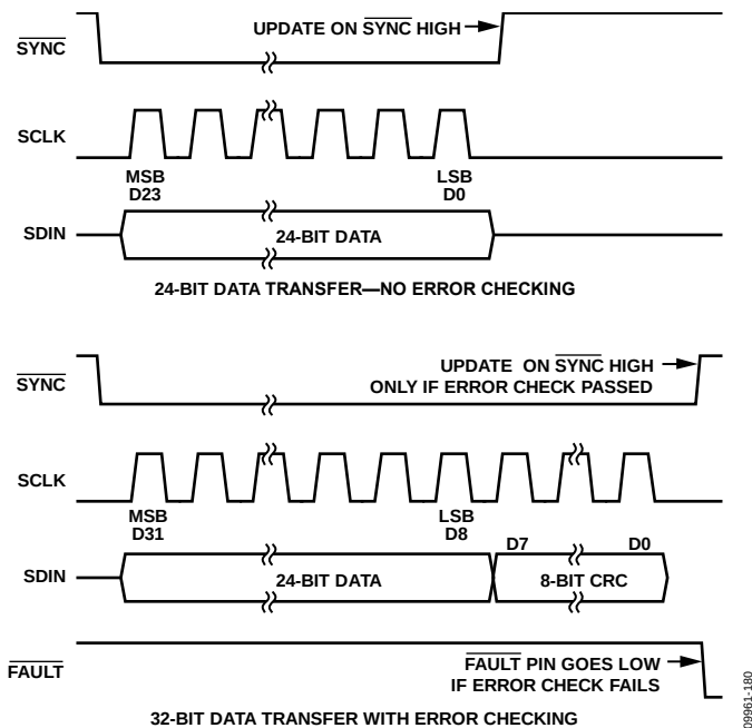
Figure 77. PEC Timing
