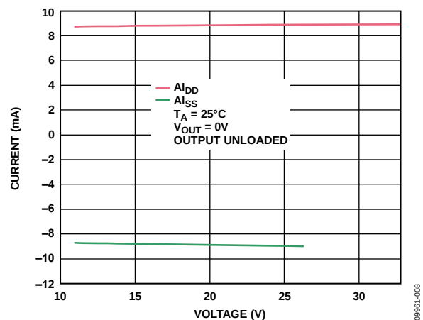
Figure 66. Supply Current ( I_{DD}/I_{SS} ) vs. Supply Voltage ( AV_{DD}/AV_{SS} )
