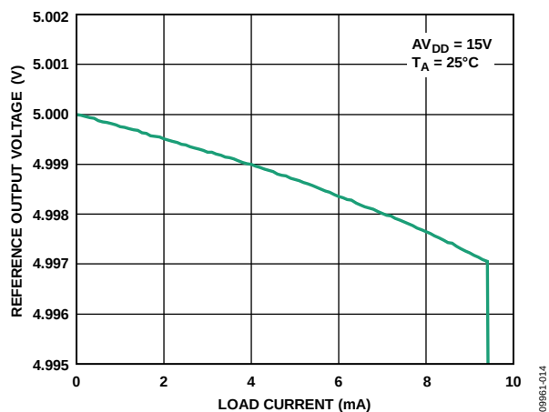
Figure 63. REFOUT Voltage vs. Load Current
