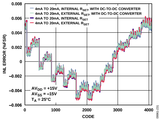
Figure 32. Integral Nonlinearity Error vs. DAC Code
