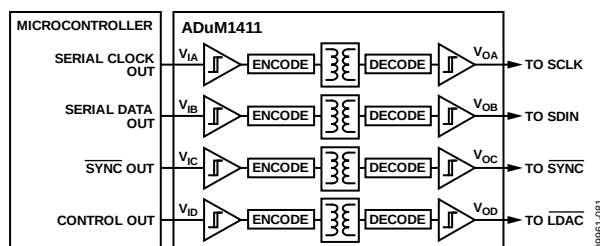
Figure 86. 4-Channel Isolated Interface to the AD5735
