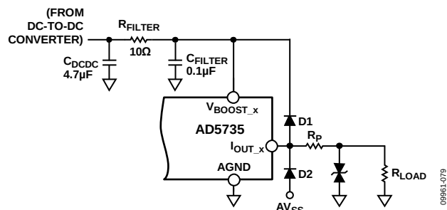
Figure 84. Output Transient Voltage Protection
