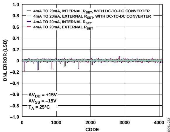
Figure 33. Differential Nonlinearity Error vs. DAC Code
