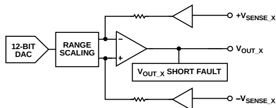
Figure 71. Voltage Output
