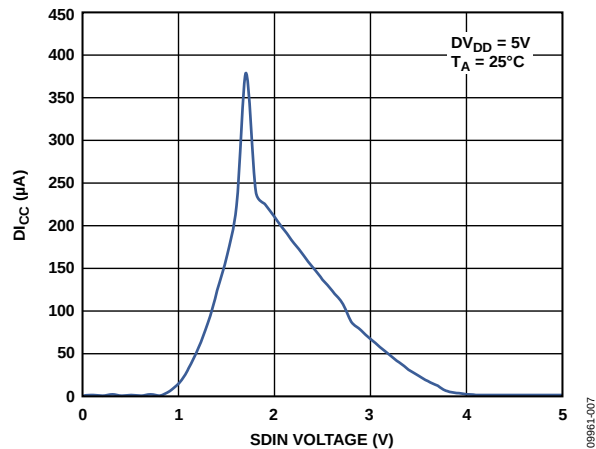
Figure 65. D_{LCC} vs. Logic Input Voltage
