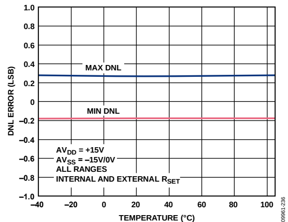
Figure 37. Differential Nonlinearity Error vs. Temperature
