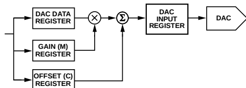
Figure 76. Digital Offset and Gain Control
