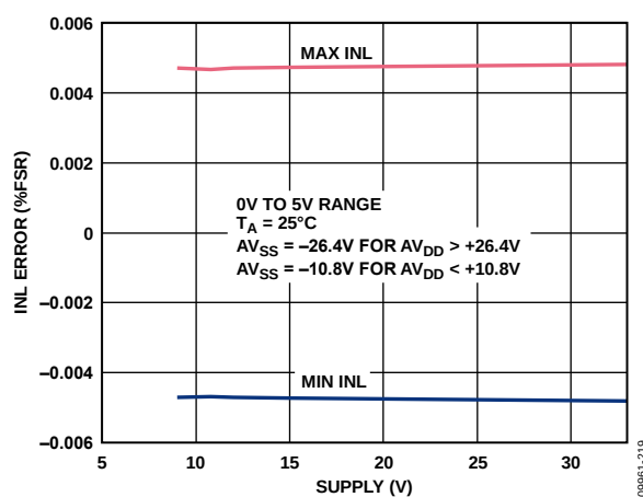
Figure 20. Integral Nonlinearity Error vs. Supply
