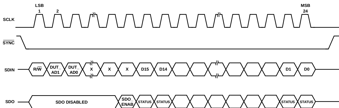
Figure 6. Status Readback During Write, Timing Diagram
