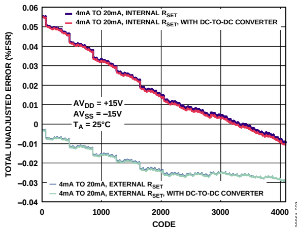
Figure 34. Total Unadjusted Error vs. DAC Code
