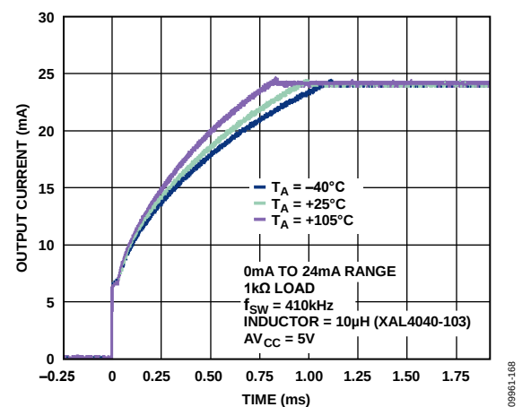
Figure 49. Output Current Settling Time with DC-to-DC Converter over Temperature (See Figure 78)
