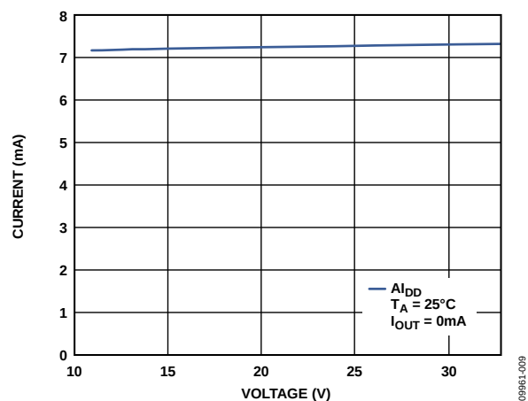
Figure 67. Supply Current ( I_{DD} ) vs. Supply Voltage ( AV_{DD} )
