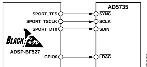
Figure 85. AD5735-to-ADSP-BF527 SPORT Interface
