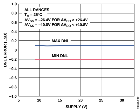
Figure 43. Differential Nonlinearity Error vs. Supply
