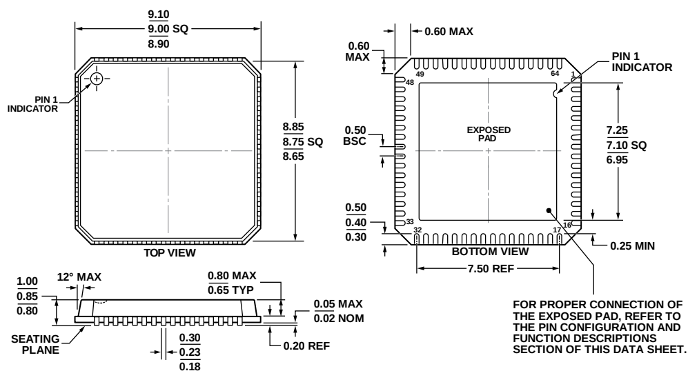
Figure 87. 64-Lead Lead Frame Chip Scale Package [LFCSP_VQ]
