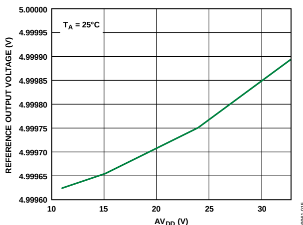
Figure 64. REFOUT Voltage vs. AV_{DD}
