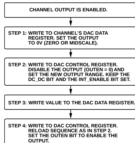
Figure 75. Programming Sequence to Change the Output Range
