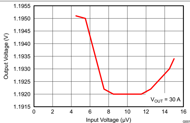
Figure 31. Line Regulation
