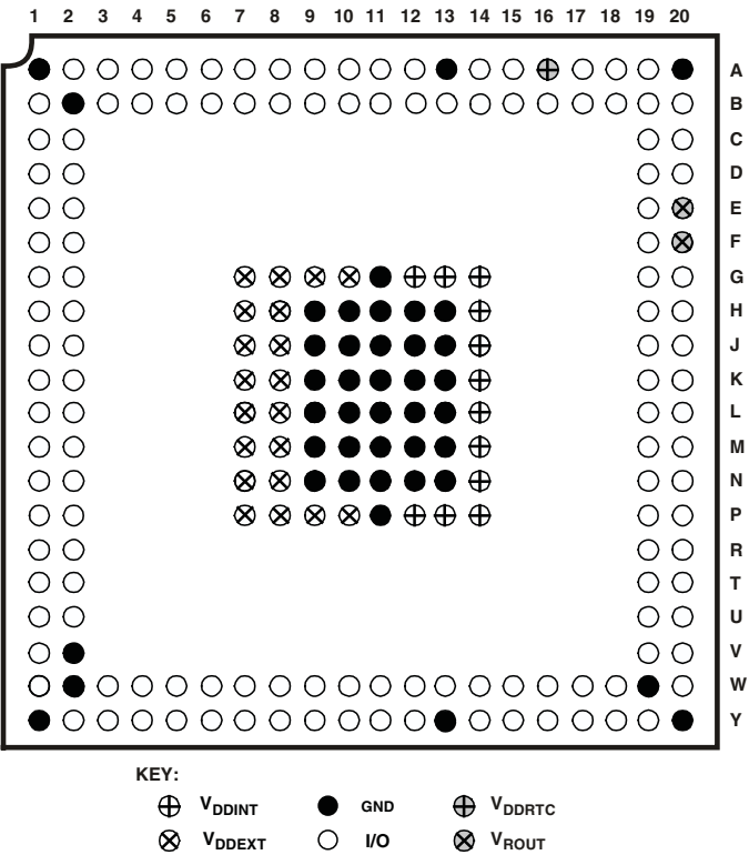
Figure 65. 208-Ball CSP_BGA Configuration (Top View)
