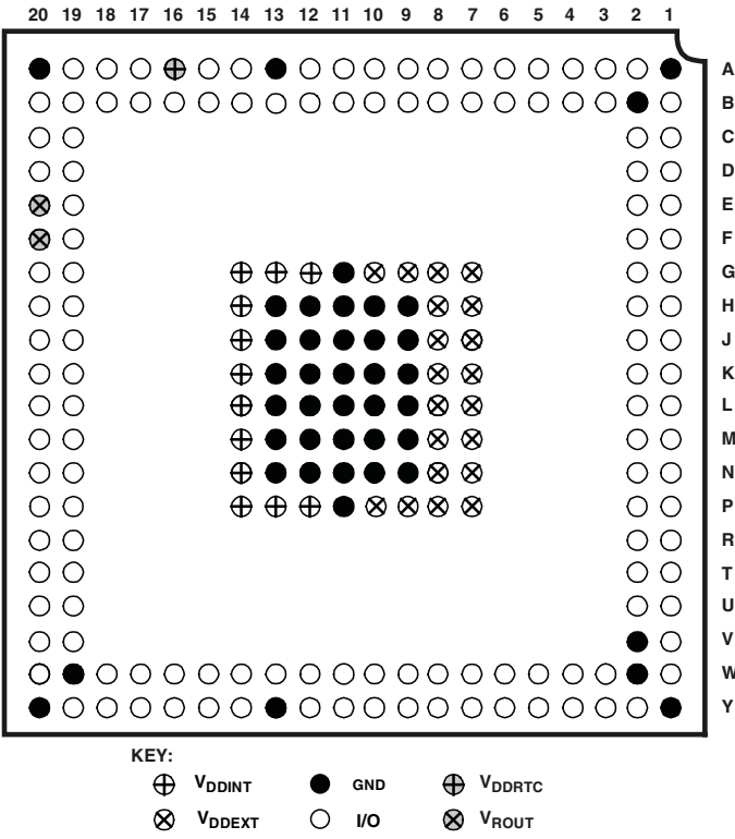
Figure 66. 208-Ball CSP_BGA Configuration (Bottom View)
